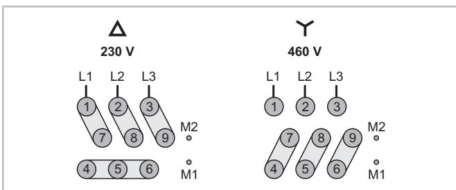
Fig. 35: Direct-on-line start connection options of the dual voltage 9-lead motor
