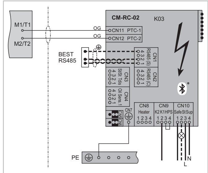
Fig. 44: Electrical connection of the CM-RC-02 in protection mode, the temperature measuring circuit (thin cables) is delivered wired. Cables shown with thick lines: required electrical connections, dashed lines: optional connection options
