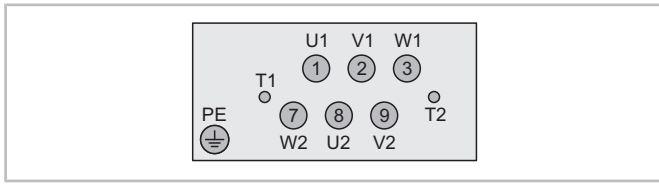
Fig. 38: Terminals and internally connected motor windings
