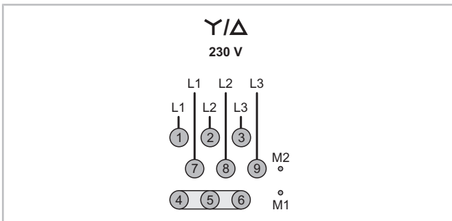
Fig. 34: Connection of the dual voltage 9-lead motor as a switchable motor
