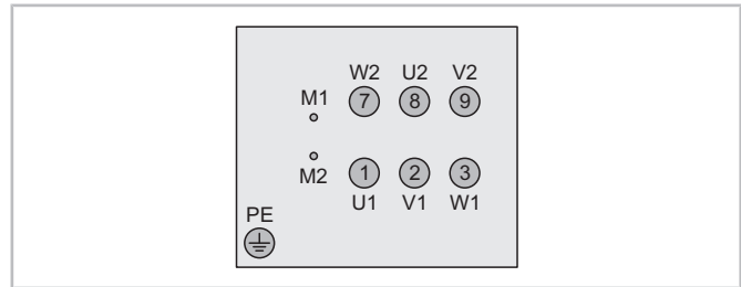
Fig. 30: Terminals and internally connected motor windings
