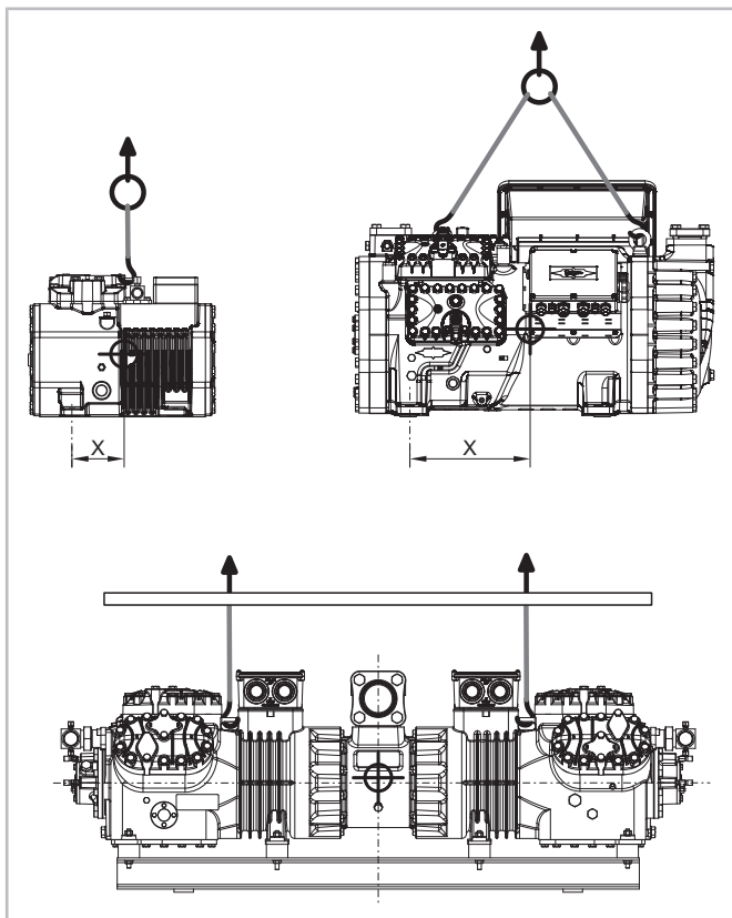
Fig. 11: Lifting the compressor; the figure shows examples. X is the deviation from the centre of gravity measured from the bore in the base on the motor side of the compressor towards the centre of the compressor. See next chapter.
