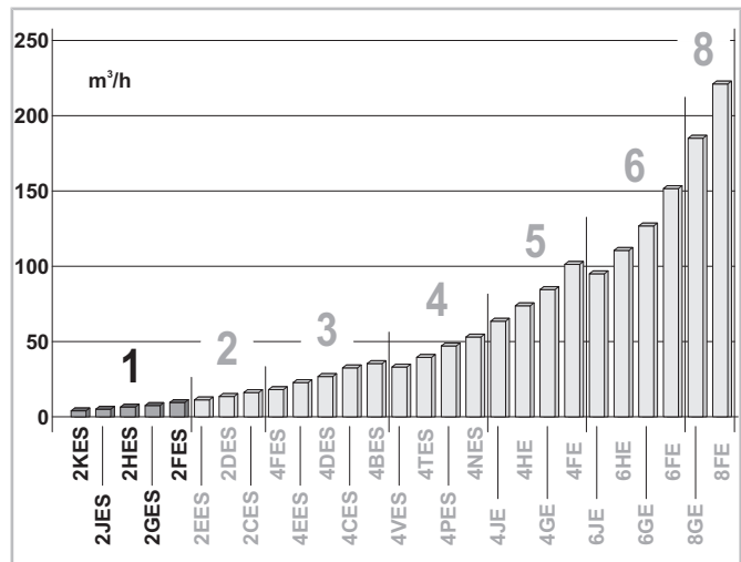
Fig. 7: Compressor overview: Displacement volumes at 50 Hz, the available compressor models are shown in dark grey.
