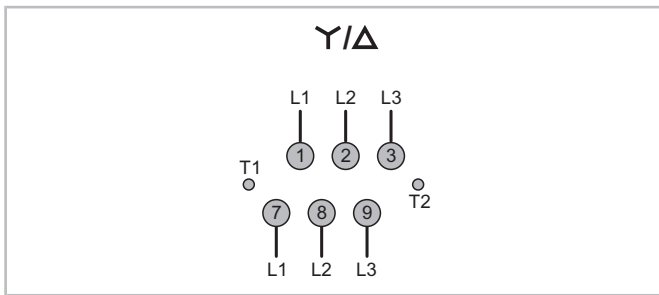
Fig. 39: Connection of the star-delta motor
