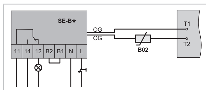
Fig. 42: Temperature measuring circuit with SE-B*
