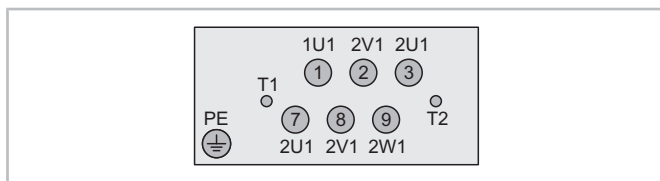
Fig. 36: Terminals and internally connected motor windings
