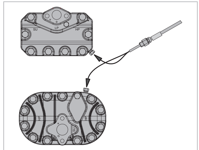
Fig. 14: With start unloading, mount the temperature sensor directly on the SU cylinder head.
