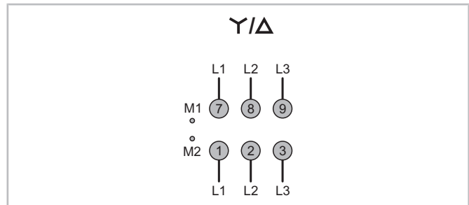
Fig. 31: Connection of the star-delta motor
