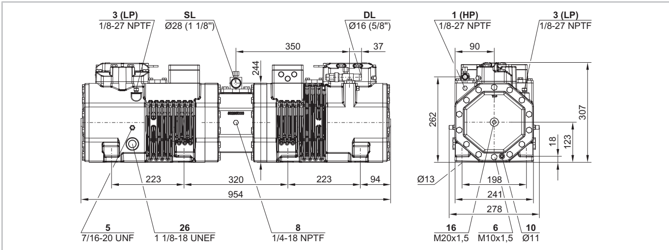
Fig. 15: Dimensions with module housing see single compressors
