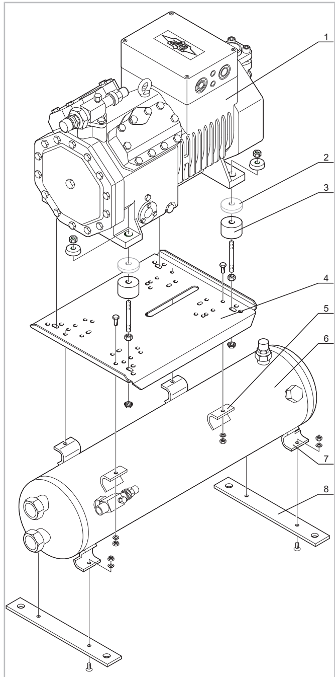
Fig. 2: Mounting with fixing plate
